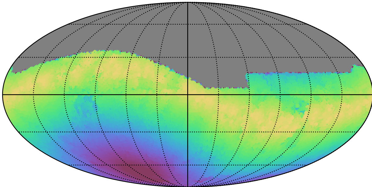
ddf_loaded_fl2_v3.4_10yrs All sky g band: Max moonDistance
