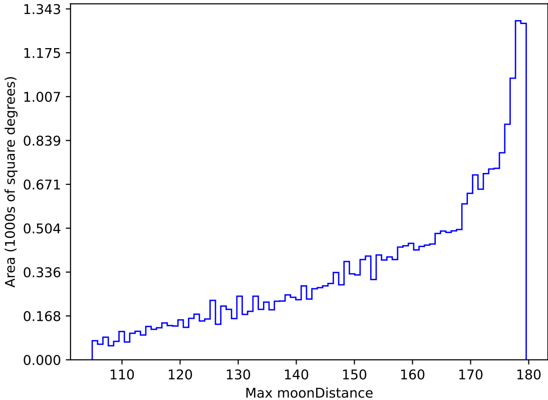
ddf_loaded_fl2_v3.4_10yrs All sky all bands: Max moonDistance
