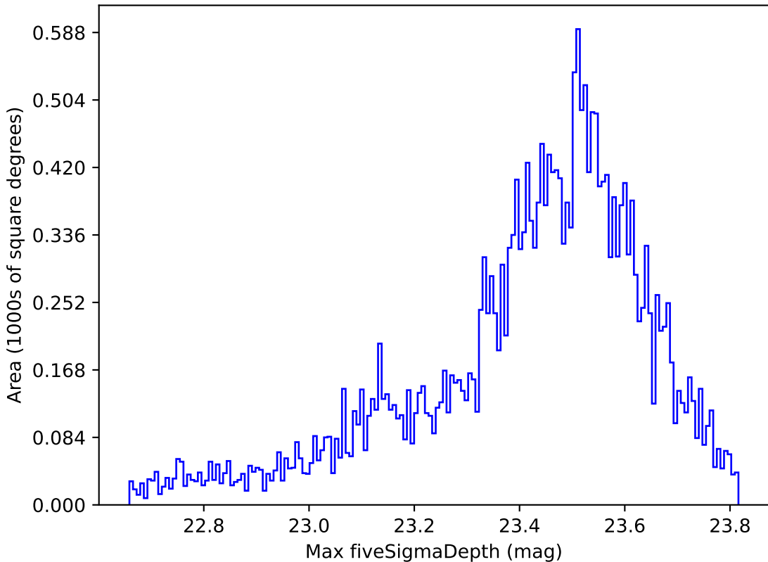
ddf_loaded_fl2_v3.4_10yrs Yr 1 z band: Max fiveSigmaDepth
