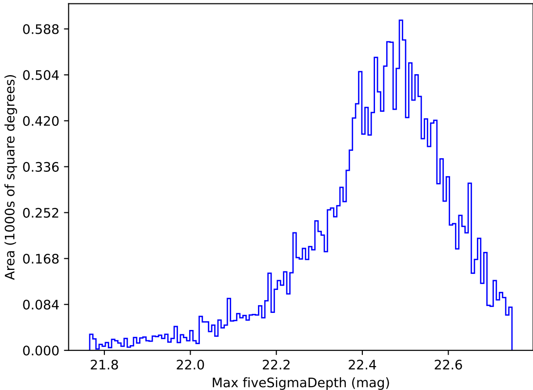
ddf_loaded_fl2_v3.4_10yrs Yr 1 y band: Max fiveSigmaDepth
