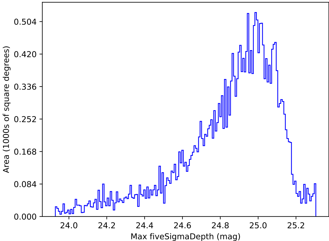
ddf_loaded_fl2_v3.4_10yrs Yr 1 g band: Max fiveSigmaDepth
