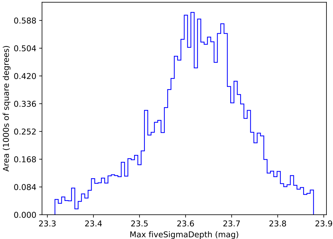
ddf_loaded_fl2_v3.4_10yrs WFD z band: Max fiveSigmaDepth
