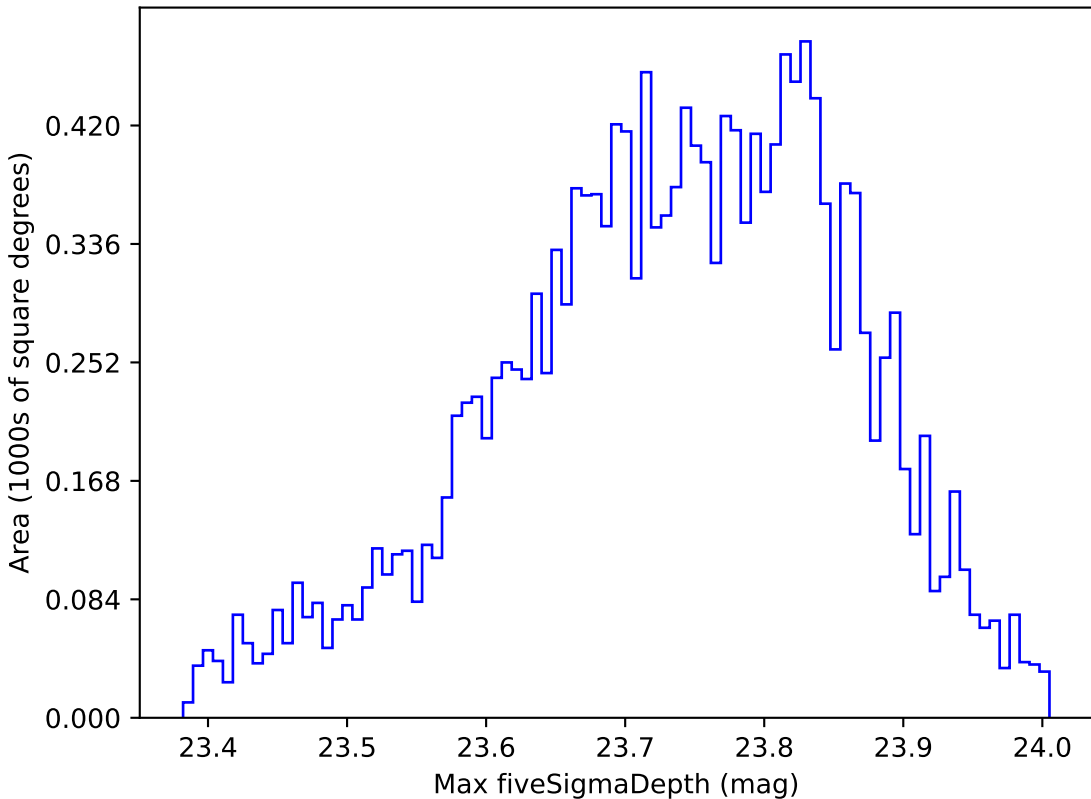
ddf_loaded_fl2_v3.4_10yrs WFD u band: Max fiveSigmaDepth
