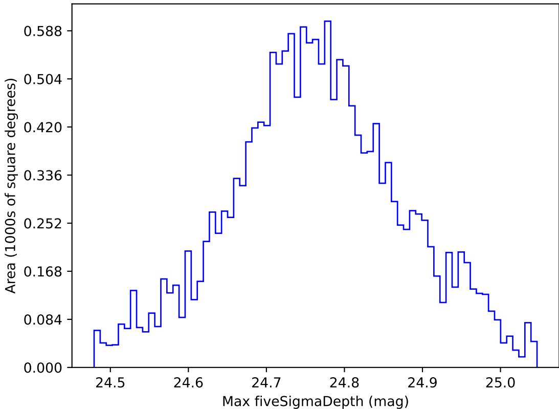
ddf_loaded_fl2_v3.4_10yrs WFD r band: Max fiveSigmaDepth
