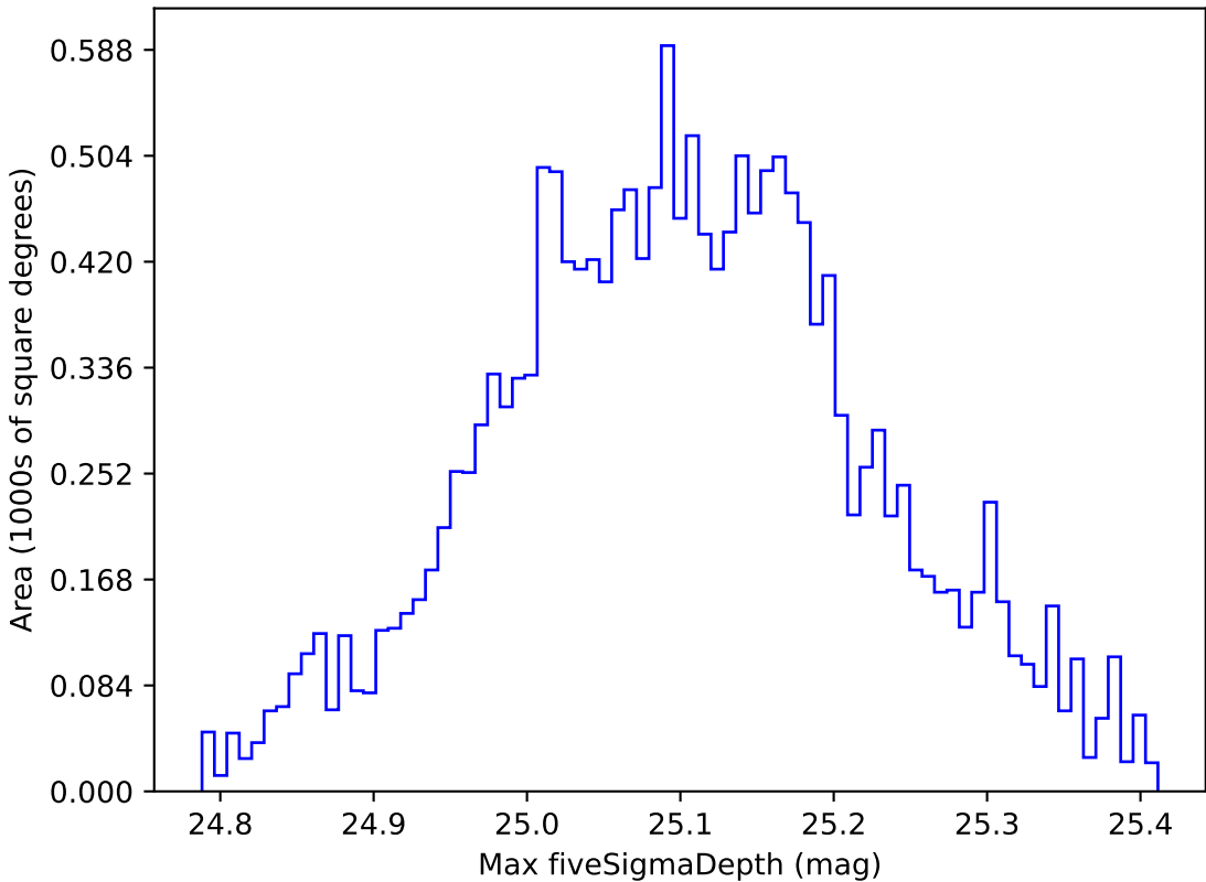
ddf_loaded_fl2_v3.4_10yrs WFD g band: Max fiveSigmaDepth
