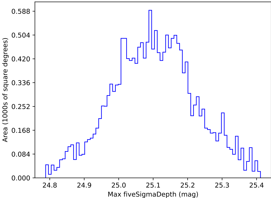
ddf_loaded_fl2_v3.4_10yrs WFD all bands: Max fiveSigmaDepth
