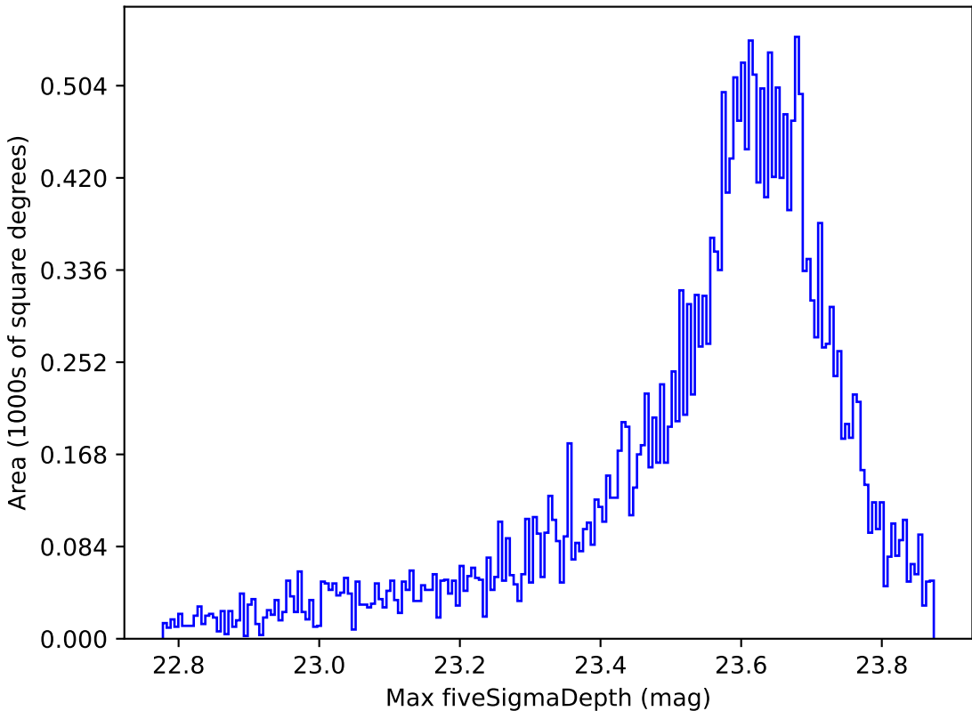
ddf_loaded_fl2_v3.4_10yrs All sky z band: Max fiveSigmaDepth
