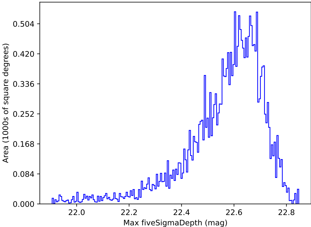
ddf_loaded_fl2_v3.4_10yrs All sky y band: Max fiveSigmaDepth
