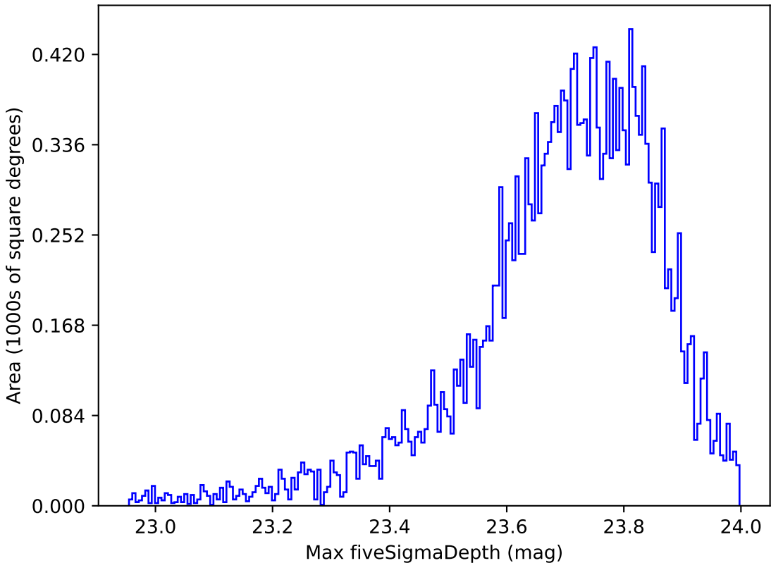
ddf_loaded_fl2_v3.4_10yrs All sky u band: Max fiveSigmaDepth
