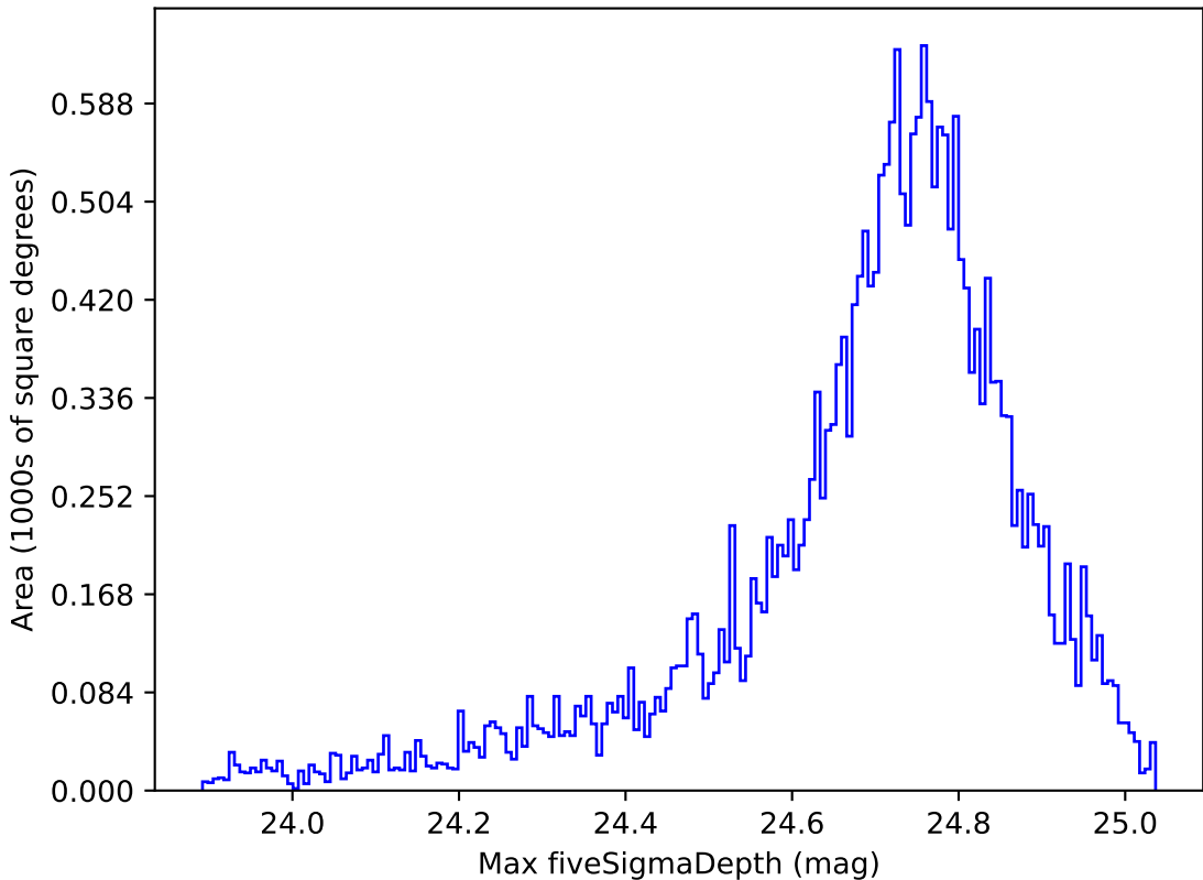
ddf_loaded_fl2_v3.4_10yrs All sky r band: Max fiveSigmaDepth
