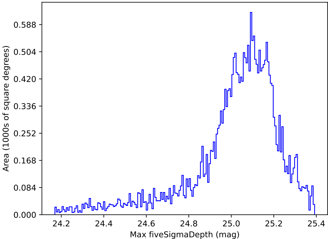
ddf_loaded_fl2_v3.4_10yrs All sky g band: Max fiveSigmaDepth
