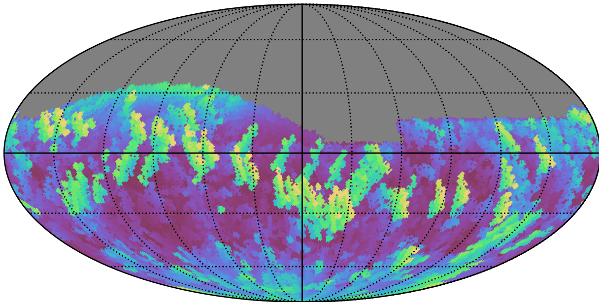
ddf_loaded_fl2_v3.4_10yrs Yr 1 z band: Max airmass
