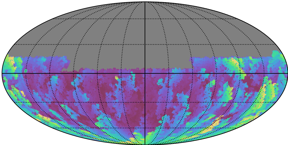
ddf_loaded_fl2_v3.4_10yrs Yr 1 u band: Max airmass
