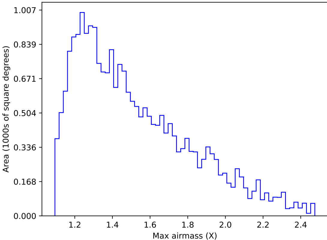
ddf_loaded_fl2_v3.4_10yrs Yr 1 u band: Max airmass
