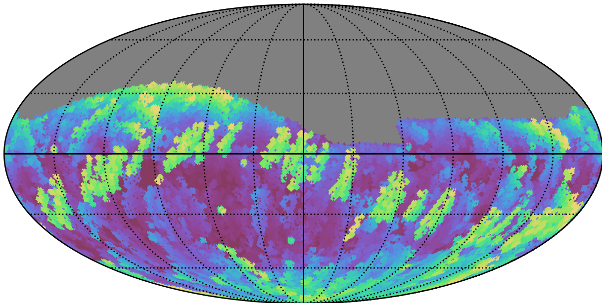
ddf_loaded_fl2_v3.4_10yrs Yr 1 r band: Max airmass
