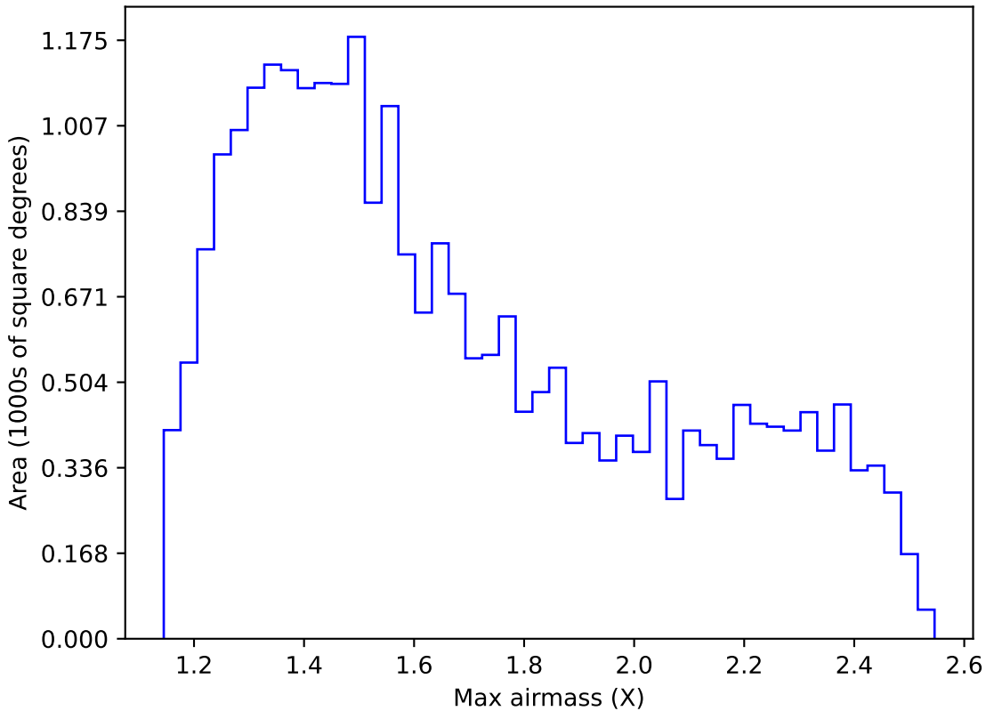
ddf_loaded_fl2_v3.4_10yrs Yr 1 r band: Max airmass
