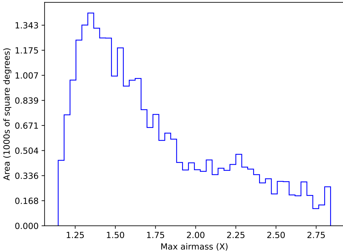
ddf_loaded_fl2_v3.4_10yrs Yr 1 i band: Max airmass
