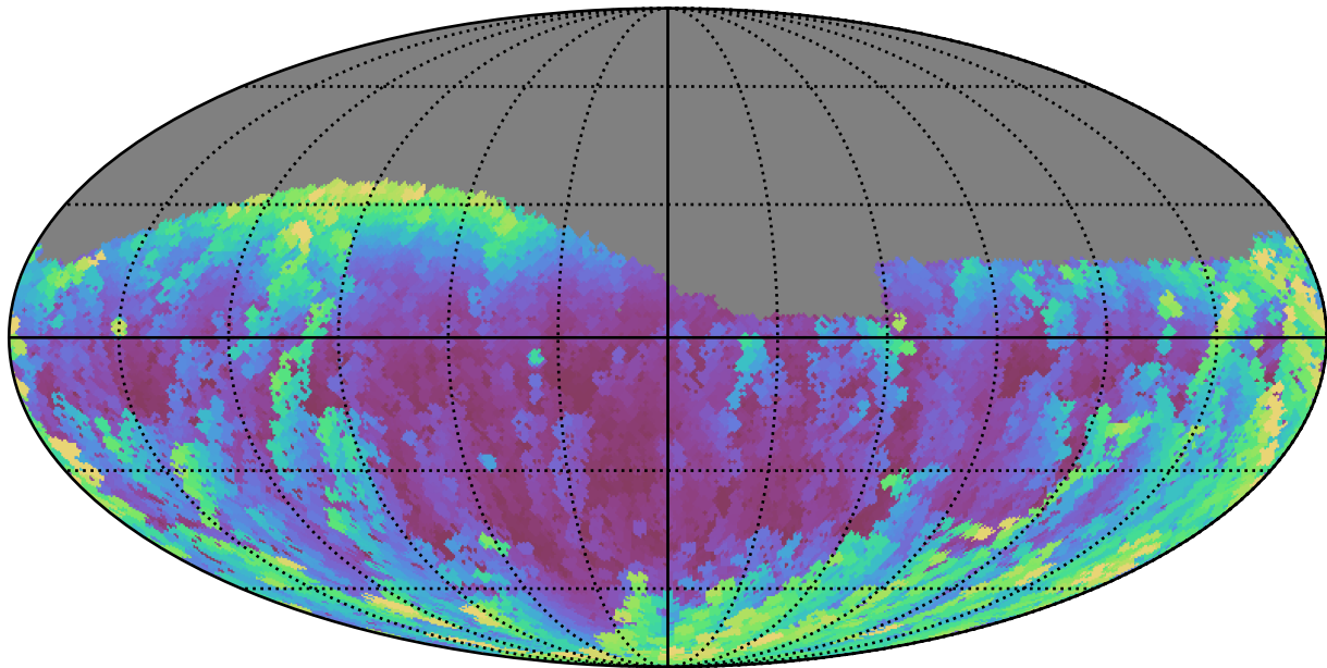
ddf_loaded_fl2_v3.4_10yrs Yr 1 g band: Max airmass
