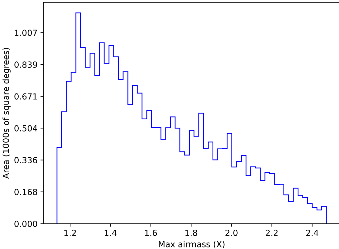
ddf_loaded_fl2_v3.4_10yrs Yr 1 g band: Max airmass
