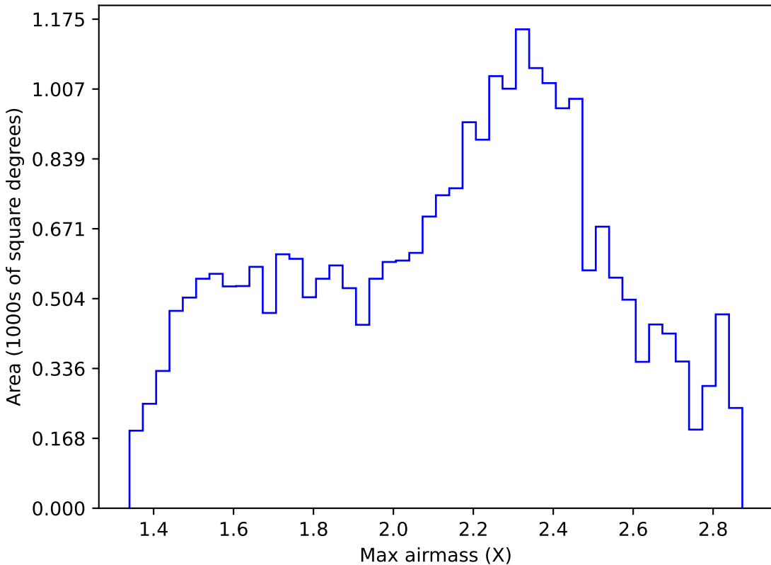
ddf_loaded_fl2_v3.4_10yrs Yr 1 all bands: Max airmass
