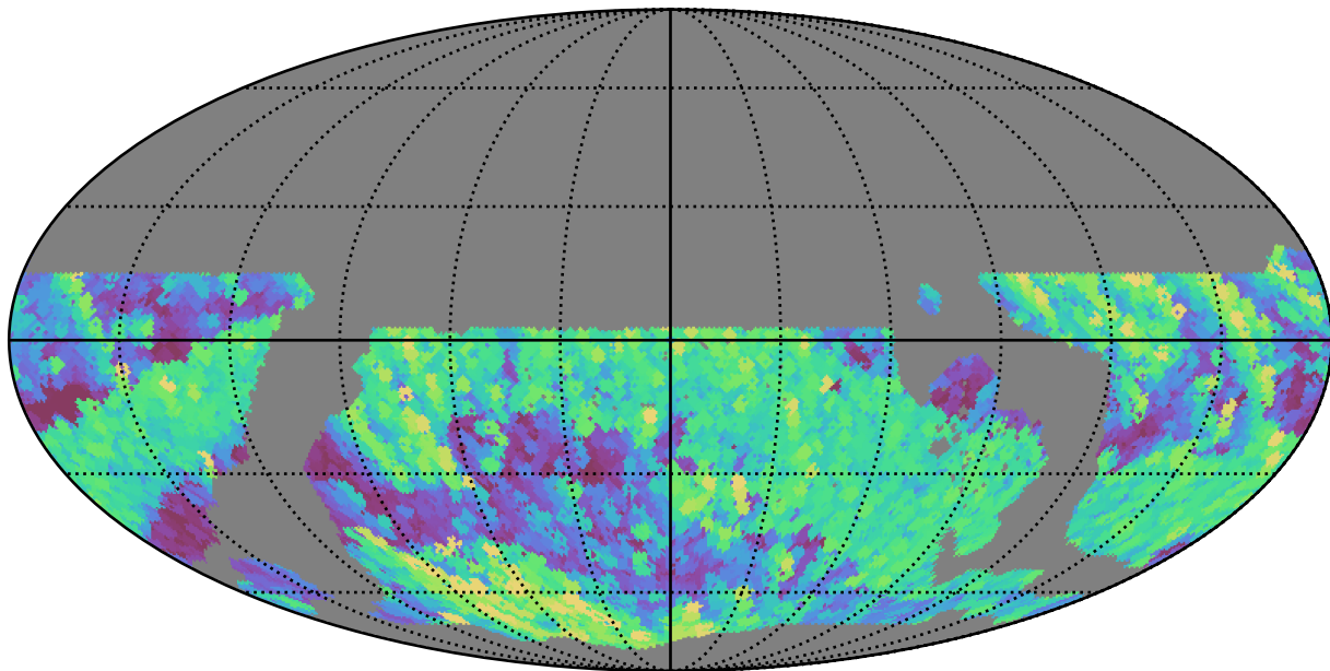
ddf_loaded_fl2_v3.4_10yrs WFD r band: Max airmass
