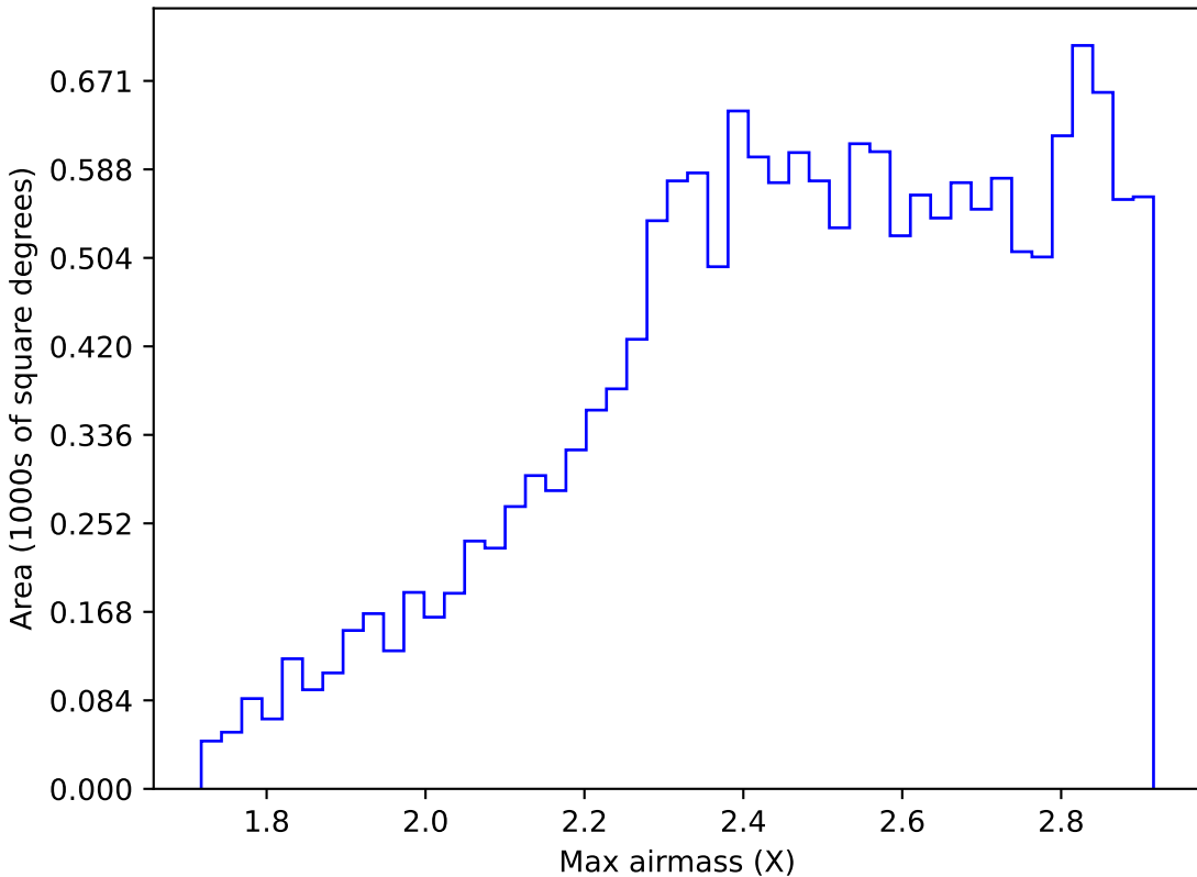
ddf_loaded_fl2_v3.4_10yrs WFD i band: Max airmass
