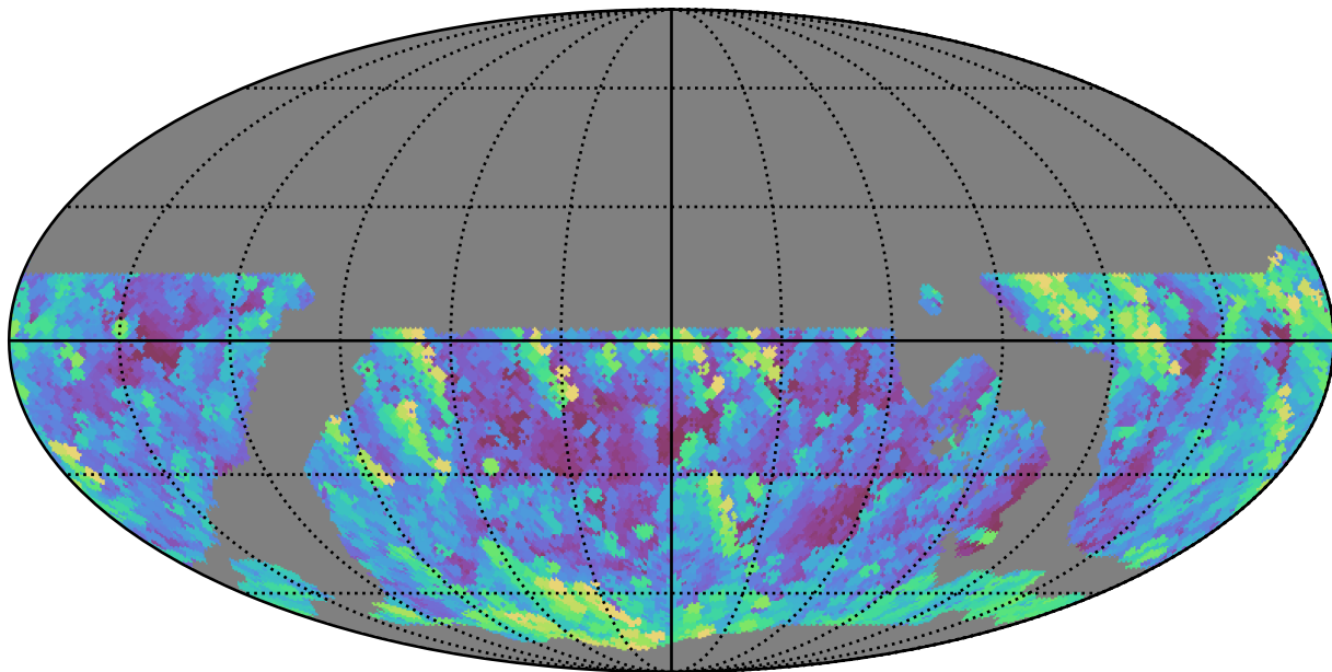
ddf_loaded_fl2_v3.4_10yrs WFD g band: Max airmass
