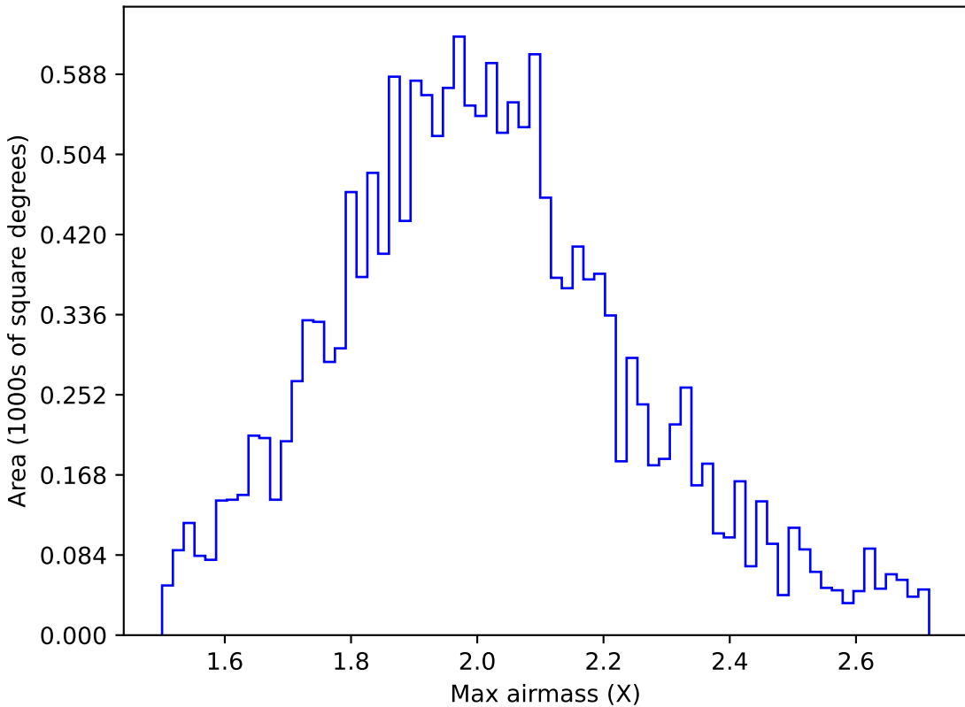
ddf_loaded_fl2_v3.4_10yrs WFD g band: Max airmass
