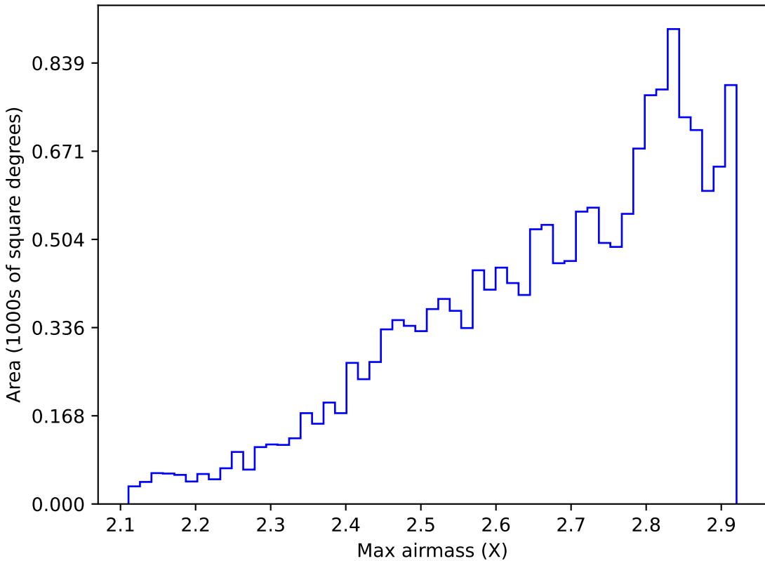
ddf_loaded_fl2_v3.4_10yrs WFD all bands: Max airmass
