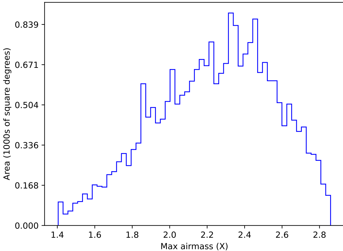
ddf_loaded_fl2_v3.4_10yrs All sky y band: Max airmass
