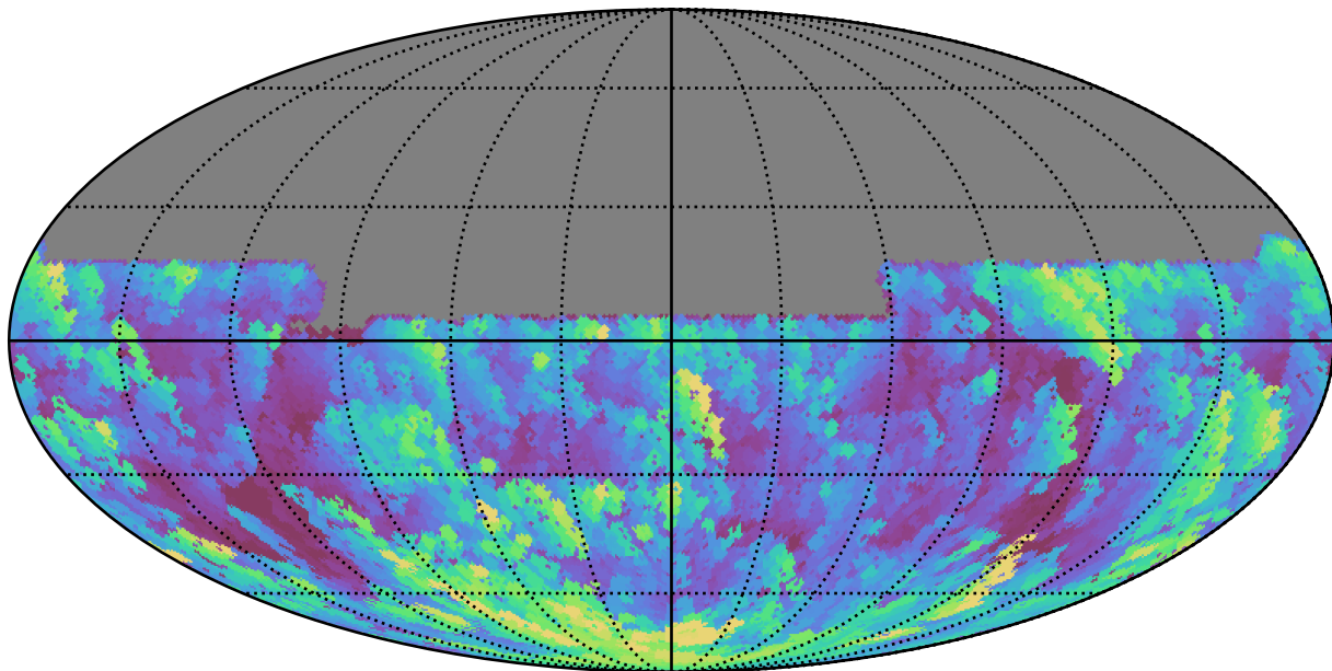
ddf_loaded_fl2_v3.4_10yrs All sky u band: Max airmass
