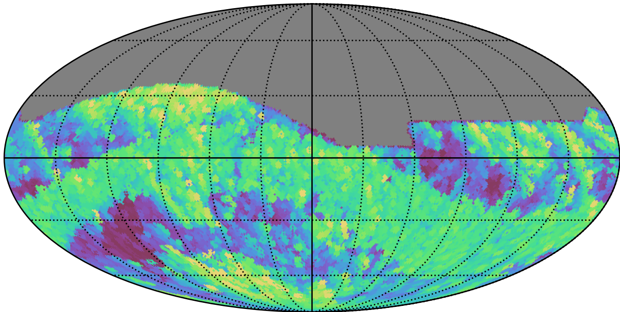
ddf_loaded_fl2_v3.4_10yrs All sky r band: Max airmass
