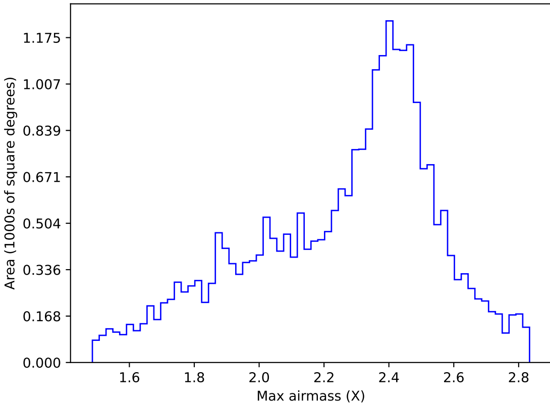
ddf_loaded_fl2_v3.4_10yrs All sky r band: Max airmass
