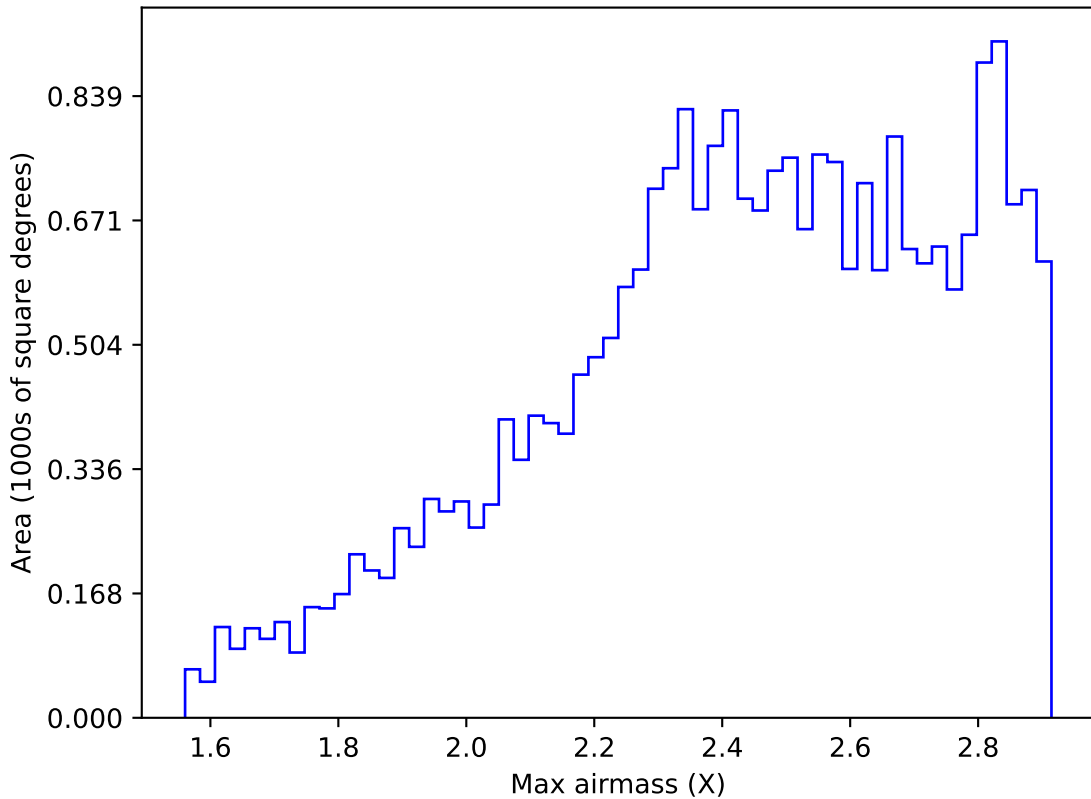
ddf_loaded_fl2_v3.4_10yrs All sky i band: Max airmass
