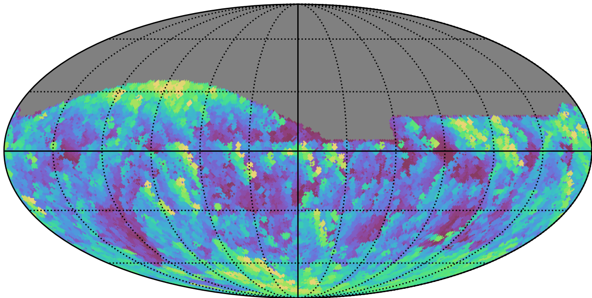
ddf_loaded_fl2_v3.4_10yrs All sky g band: Max airmass
