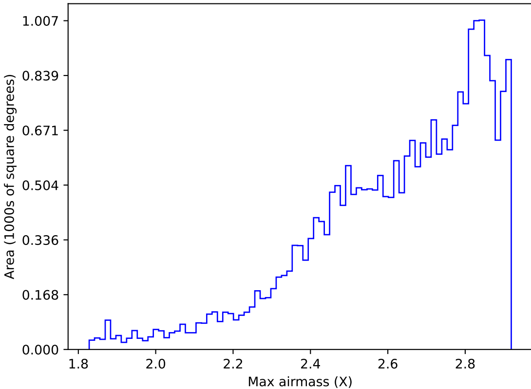
ddf_loaded_fl2_v3.4_10yrs All sky all bands: Max airmass
