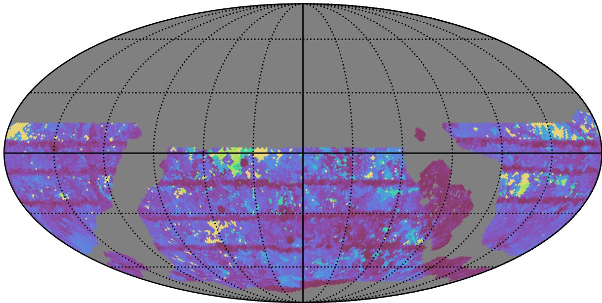
ddf_loaded_fl2_v3.4_10yrs WFD z band: Max Inter-Night Gap
