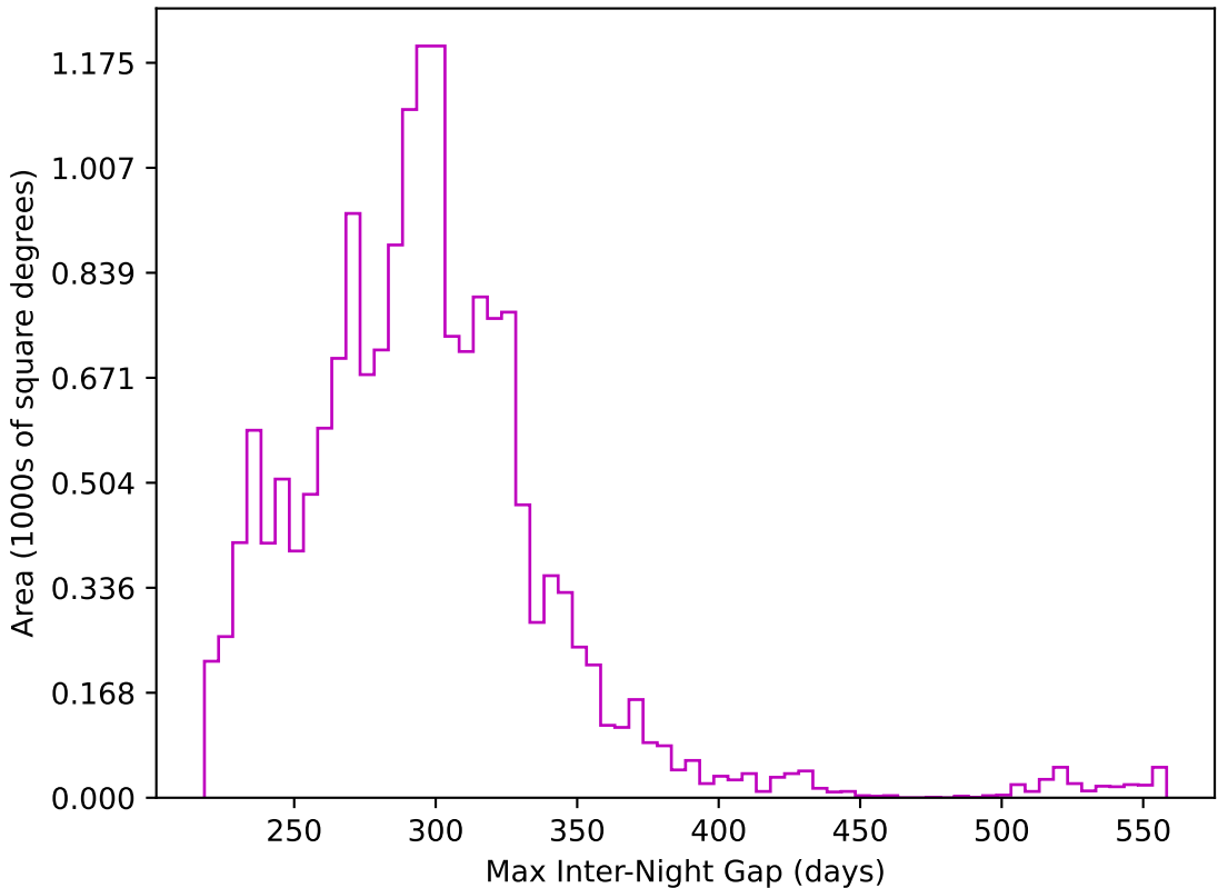
ddf_loaded_fl2_v3.4_10yrs WFD z band: Max Inter-Night Gap
