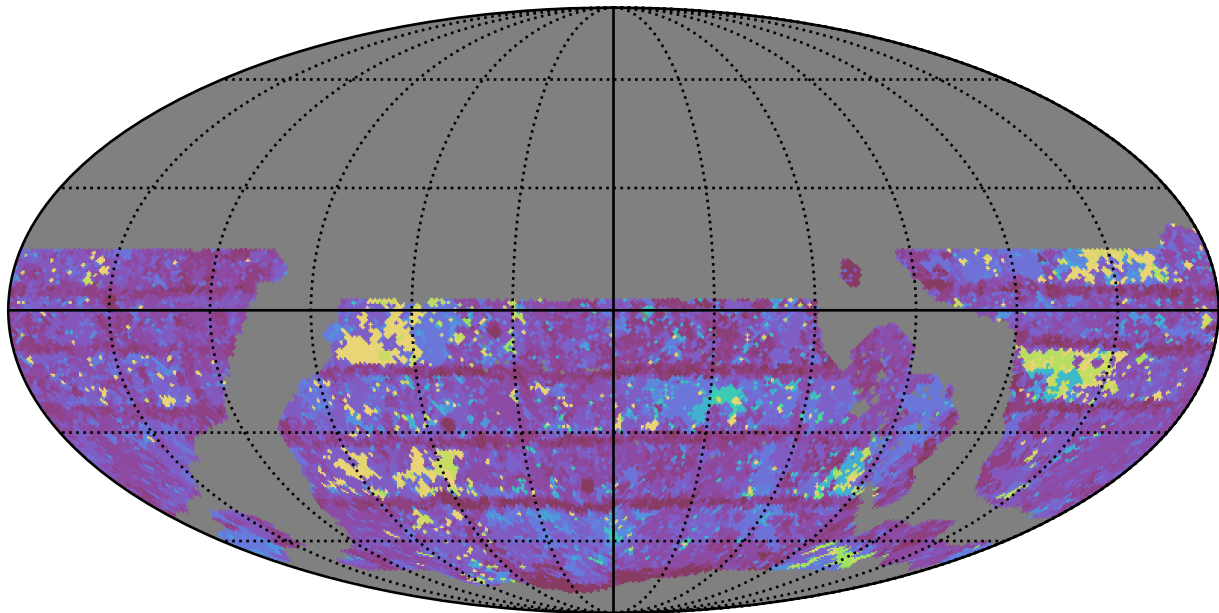
ddf_loaded_fl2_v3.4_10yrs WFD y band: Max Inter-Night Gap
