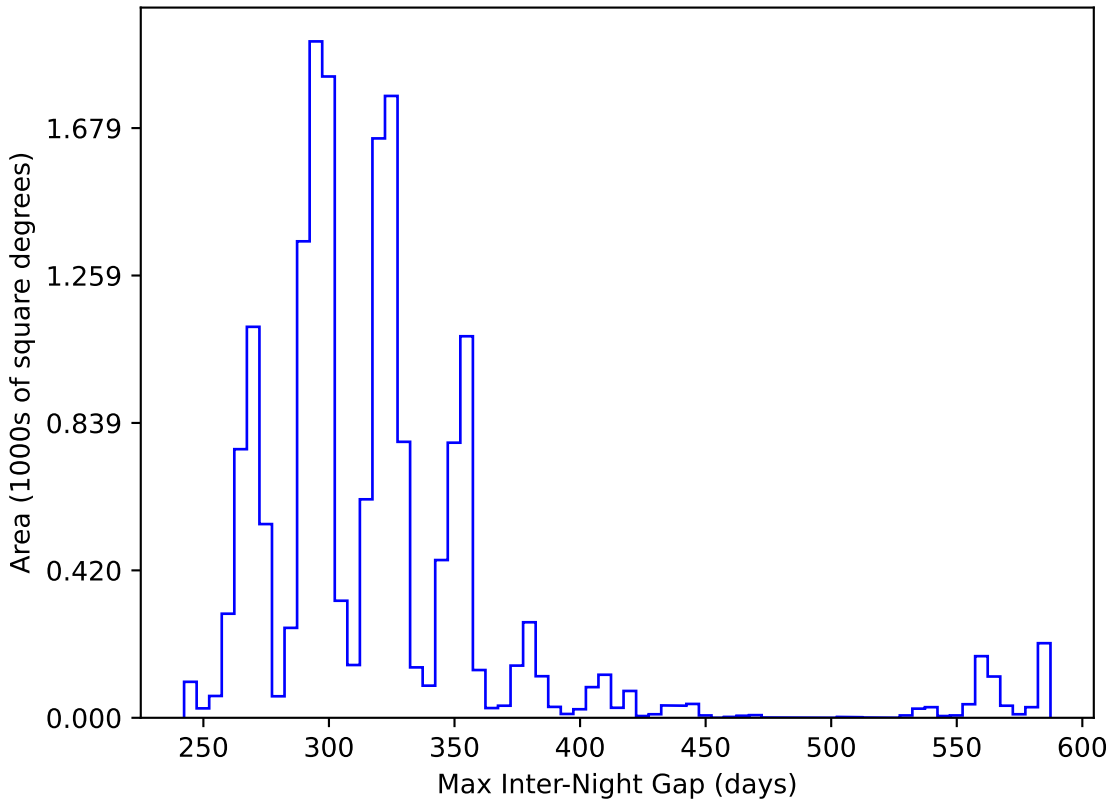
ddf_loaded_fl2_v3.4_10yrs WFD y band: Max Inter-Night Gap
