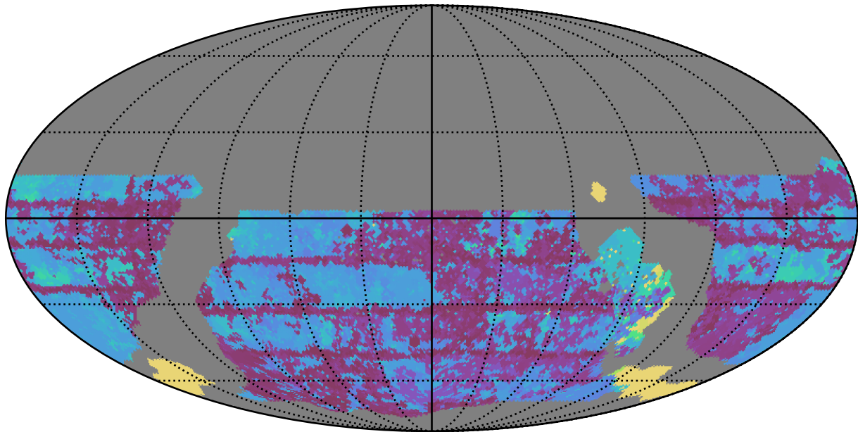
ddf_loaded_fl2_v3.4_10yrs WFD u band: Max Inter-Night Gap
