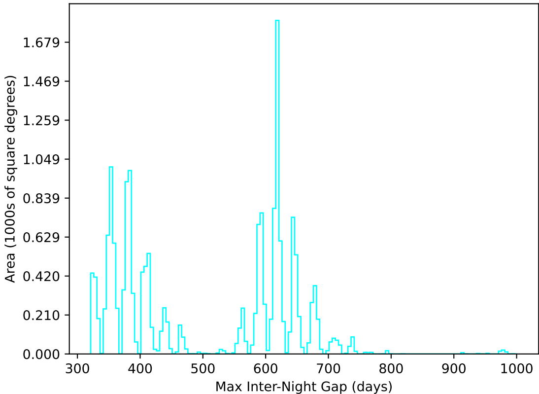
ddf_loaded_fl2_v3.4_10yrs WFD u band: Max Inter-Night Gap
