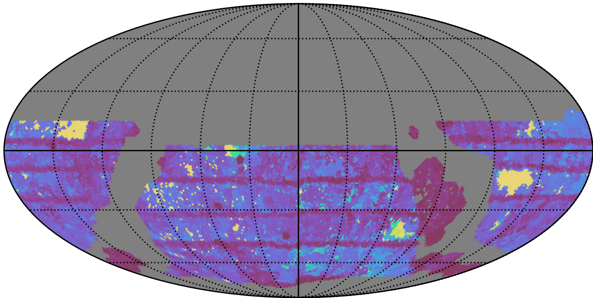
ddf_loaded_fl2_v3.4_10yrs WFD r band: Max Inter-Night Gap
