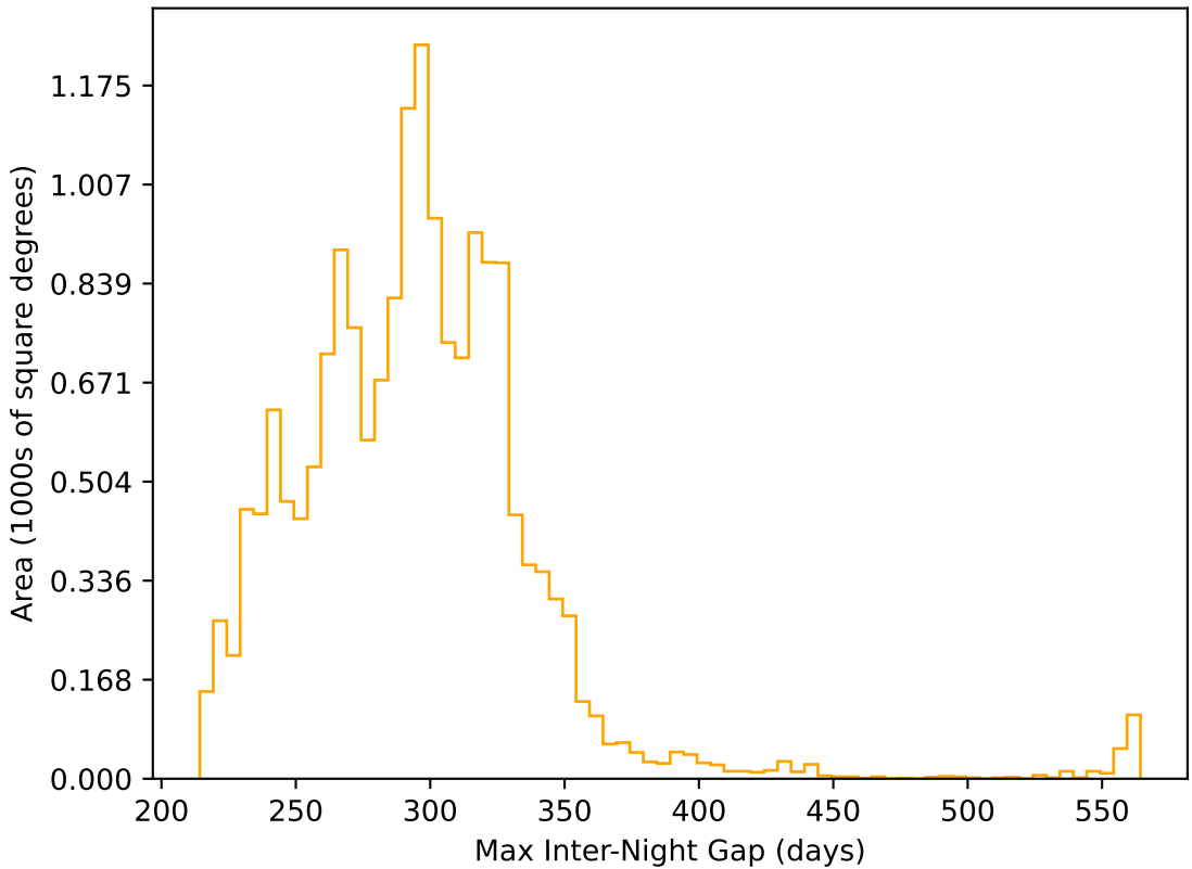
ddf_loaded_fl2_v3.4_10yrs WFD r band: Max Inter-Night Gap
