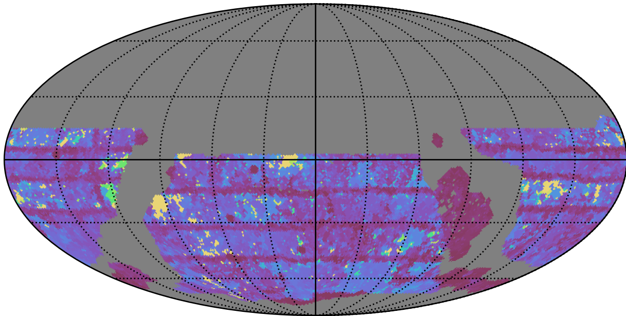
ddf_loaded_fl2_v3.4_10yrs WFD i band: Max Inter-Night Gap
