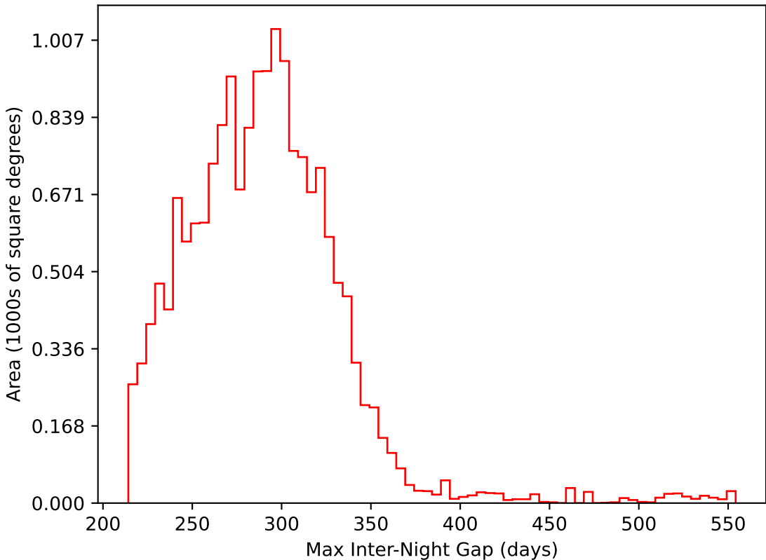
ddf_loaded_fl2_v3.4_10yrs WFD i band: Max Inter-Night Gap
