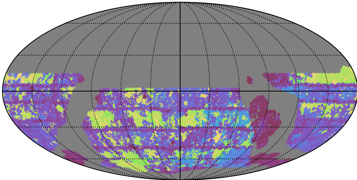
ddf_loaded_fl2_v3.4_10yrs WFD g band: Max Inter-Night Gap
