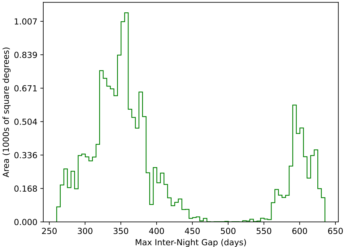
ddf_loaded_fl2_v3.4_10yrs WFD g band: Max Inter-Night Gap
