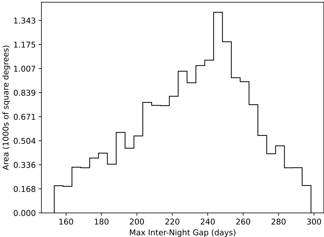
ddf_loaded_fl2_v3.4_10yrs WFD all bands: Max Inter-Night Gap
