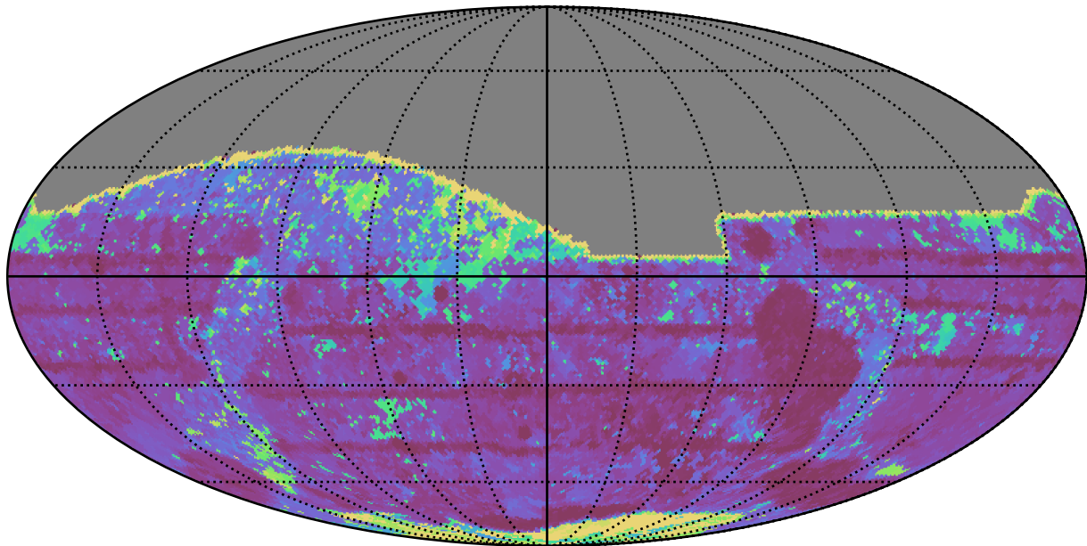
ddf_loaded_fl2_v3.4_10yrs All sky z band: Max Inter-Night Gap
